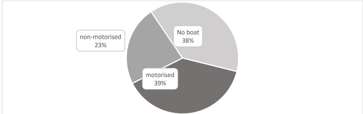
Figure 1. Overall contribution of the main boat types to total reported catch.
