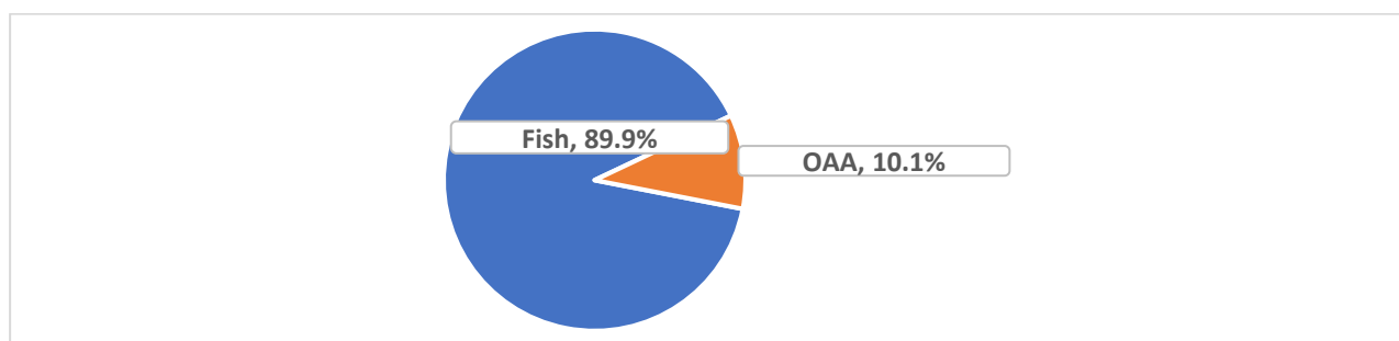
Figure 4. Catch contribution for fish and other aquatic animals.
