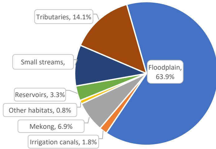
Figure 2. Overall contribution of the habitats to total reported catch, with proportion of catch for floodplain habitats.
